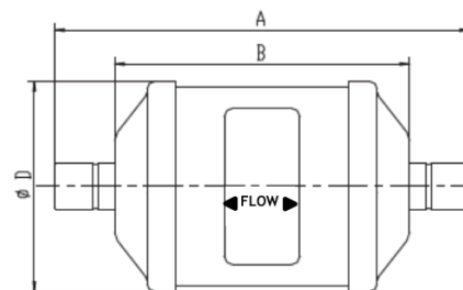
Solder Connection
