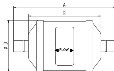
Solder Connection
